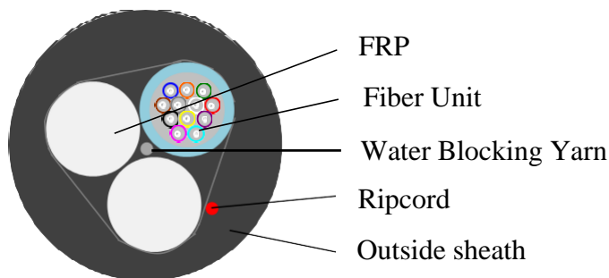
Cable Section Sketch Map
